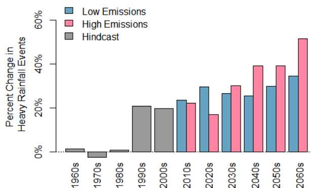
The graph shows the % increase in days with ≥ 2" rain relative to a 1960-1989 mean. High-emission projections (RCP 8.5) are in red and low-emission projections (RCP 4.5) in blue. Precipitation hindcasts are in gray. Modeled data are from Multivariate Adaptive Constructed Analogs (MACA).
