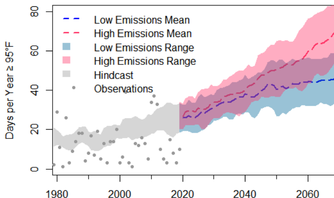
High-emissions temperature projections (RCP 8.5) are in red, and low-emission projections (RCP 4.5) in blue. Dots represent annual days ≥ 95°F, and gray shading shows temperature hindcasts. Modeled data are retrieved from Multivariate Adaptive Constructed Analogs (MACA) 5 , and observed data are from the Gridded Surface Meteorological Dataset (gridMET). 6
